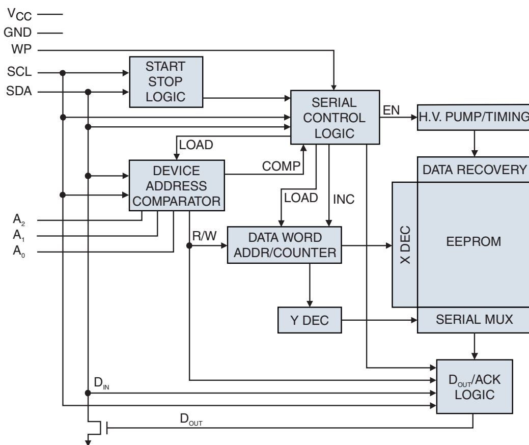
Figure 2. Block Diagram
